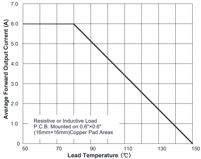
FIG.1: Io-TL Curve
